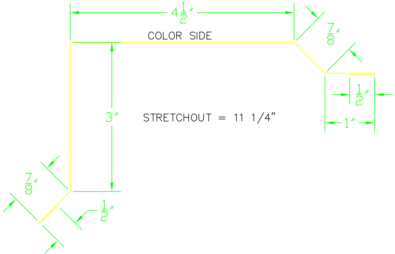
AG PANEL GABLE TRIM
