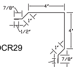
Residential Outside Corner Trim
