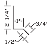
Residential Drip Cap
