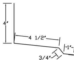
Residential Endwall Trim
