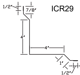
Residential Inside Corner Trim
